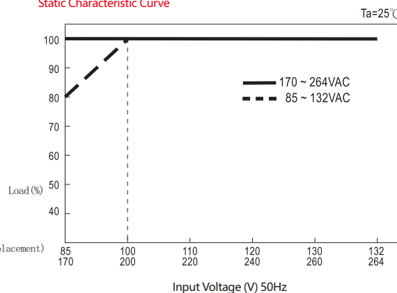
Static Characteristic Curve
