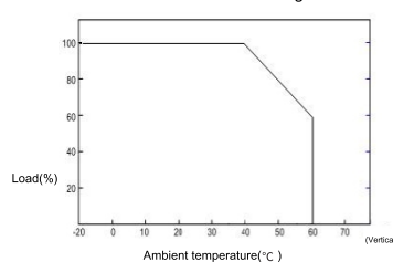
Static characteristic curve diagram
