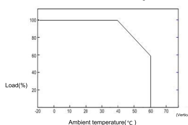
Static characteristic curve diagram
