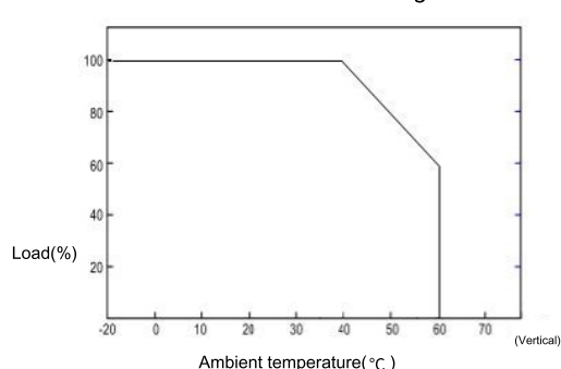
Static characteristic curve diagram
