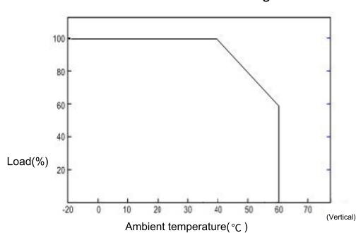
Static characteristic curve diagram
