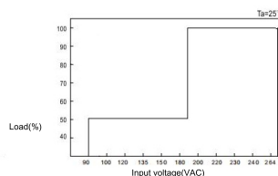
Static characteristic curve diagram
